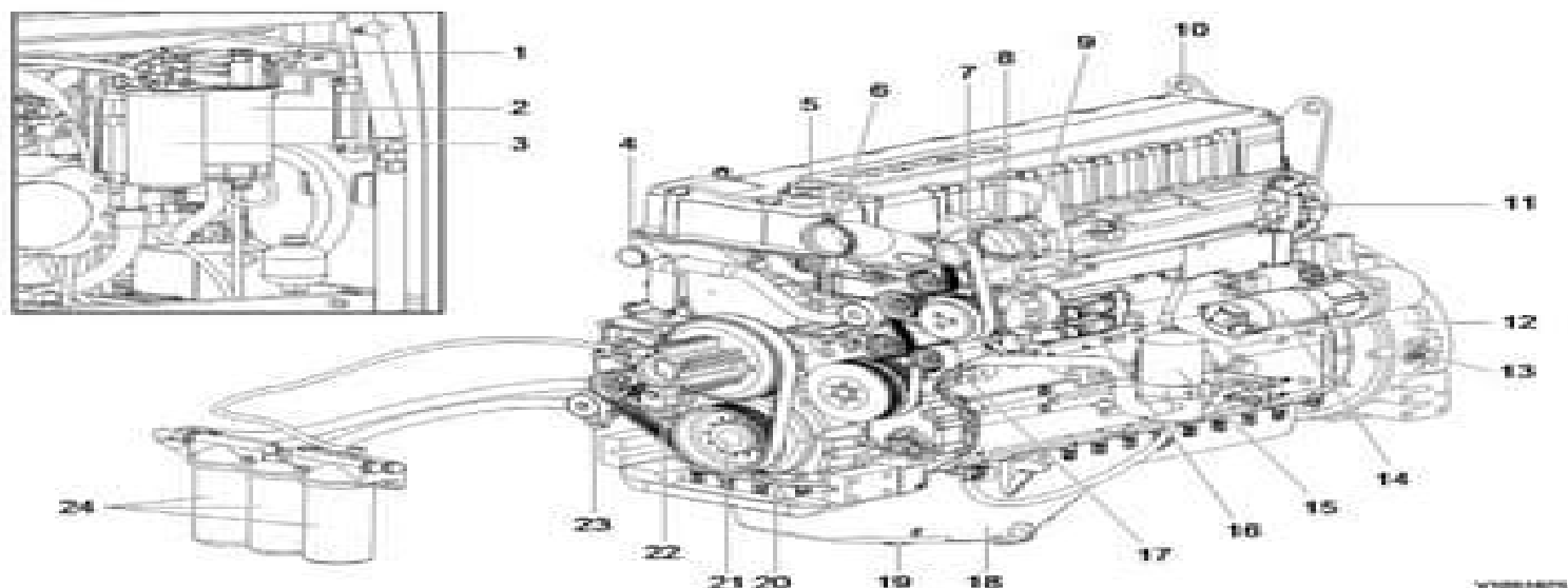
Figure 1 Engine, structure
