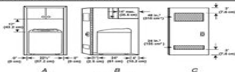
A. Front view B. Side view C. Closet door with vents
