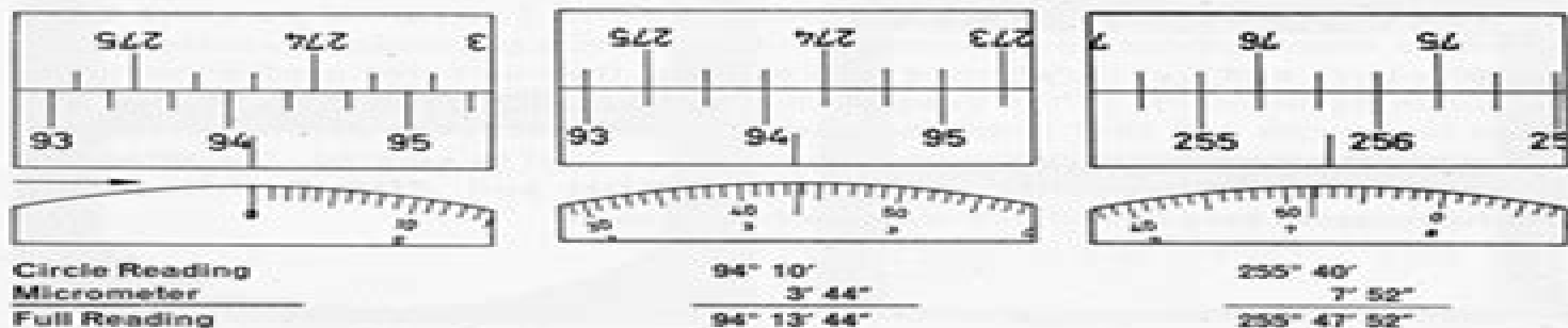
Fig. 7 Circle Reading with the Wild T2 Universal Theodolite (Horizontal or Vertical Circle)
