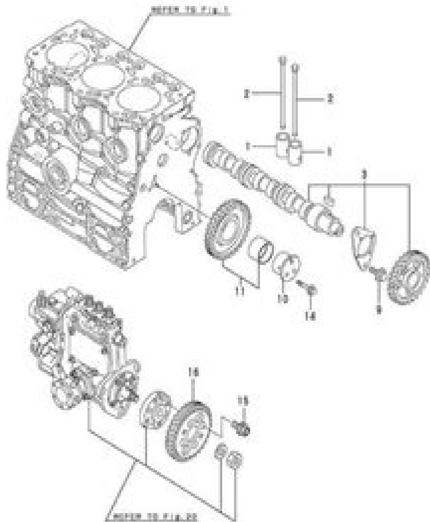
Fig.9. CAMSHAFT & DRIVING GEAR
