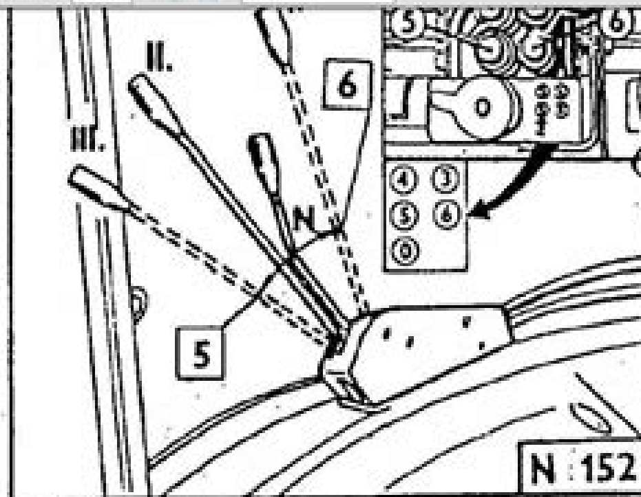
THREE-POSITION VERSION
