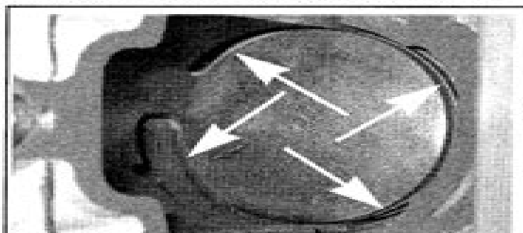
Fig. 25a The combustion chamber of a typical looper, notice the piston is far enough down the cylinder bore to reveal intake and exhaust ports
